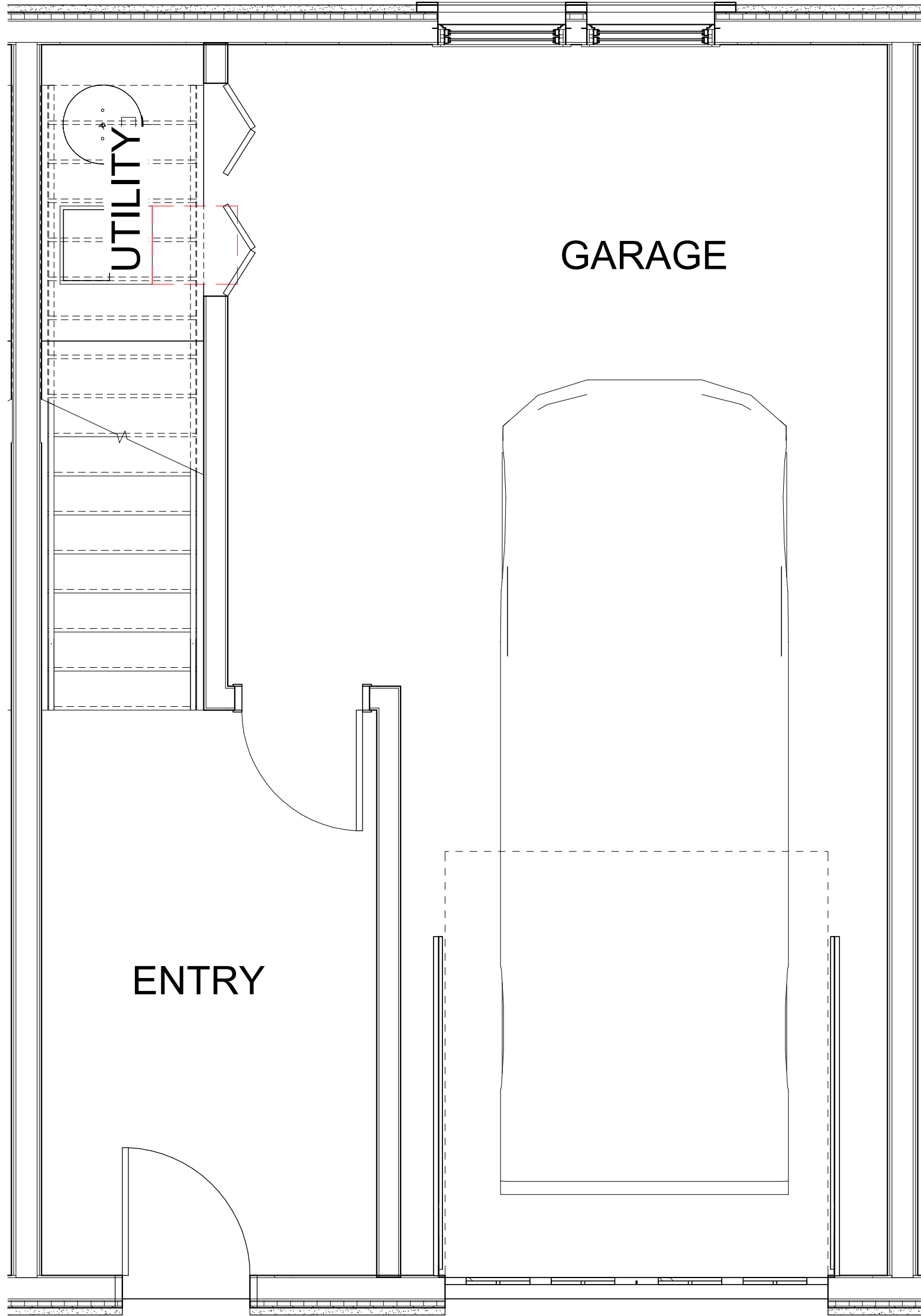
1 1-BED W/ GARAGE LEVEL 1 3/8" = 1'-0"
