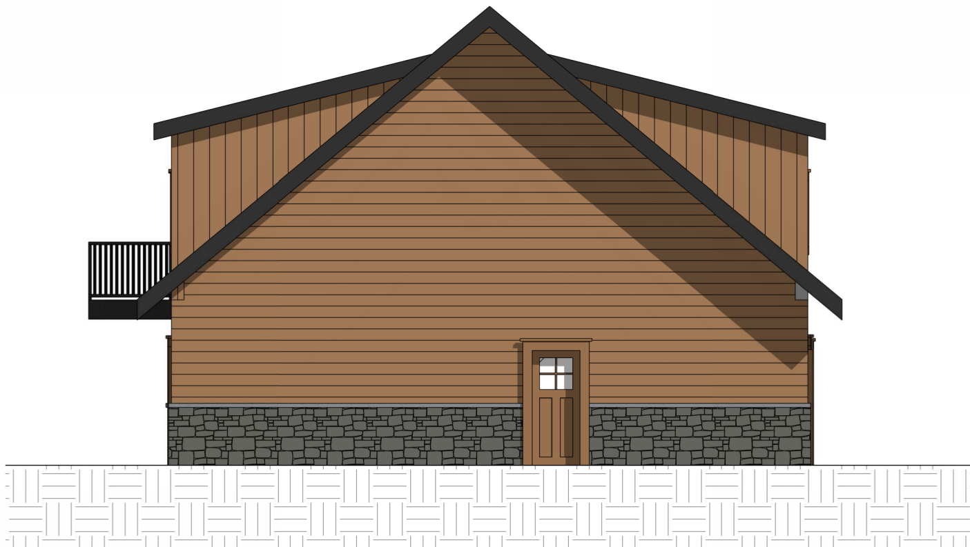
4 BUILDING 2 - LEFT 1/8" = 1'-0"
