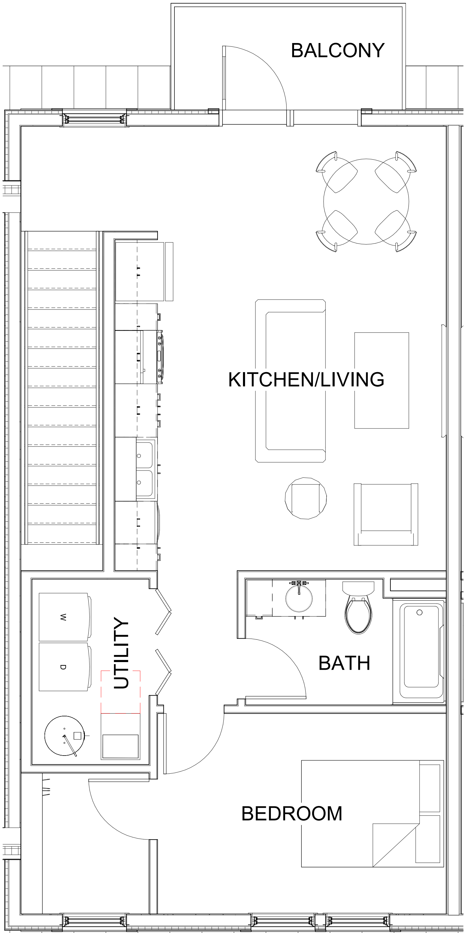
2 UPPER LEVEL 1-BED 3/8" = 1'-0"
