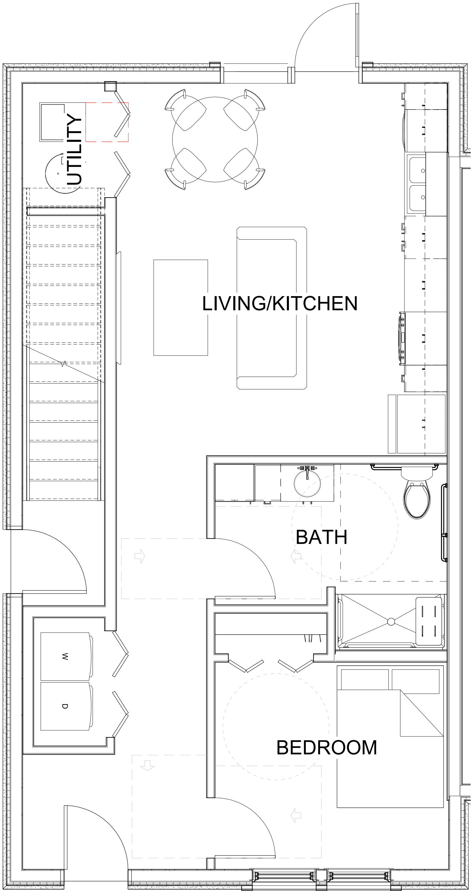
1 ADA 1-BED 3/8" = 1'-0"
