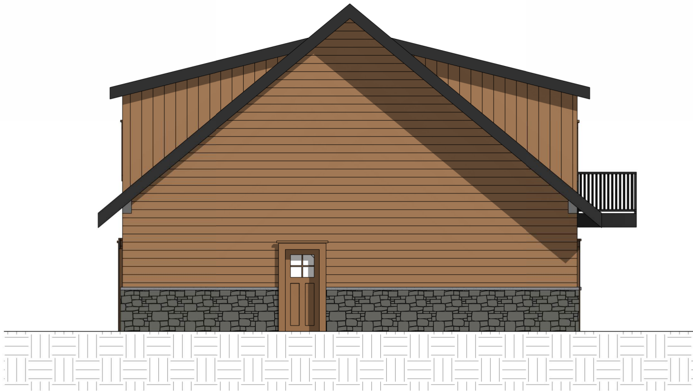
2 BUILDING 2 - RIGHT 1/8" = 1'-0"
