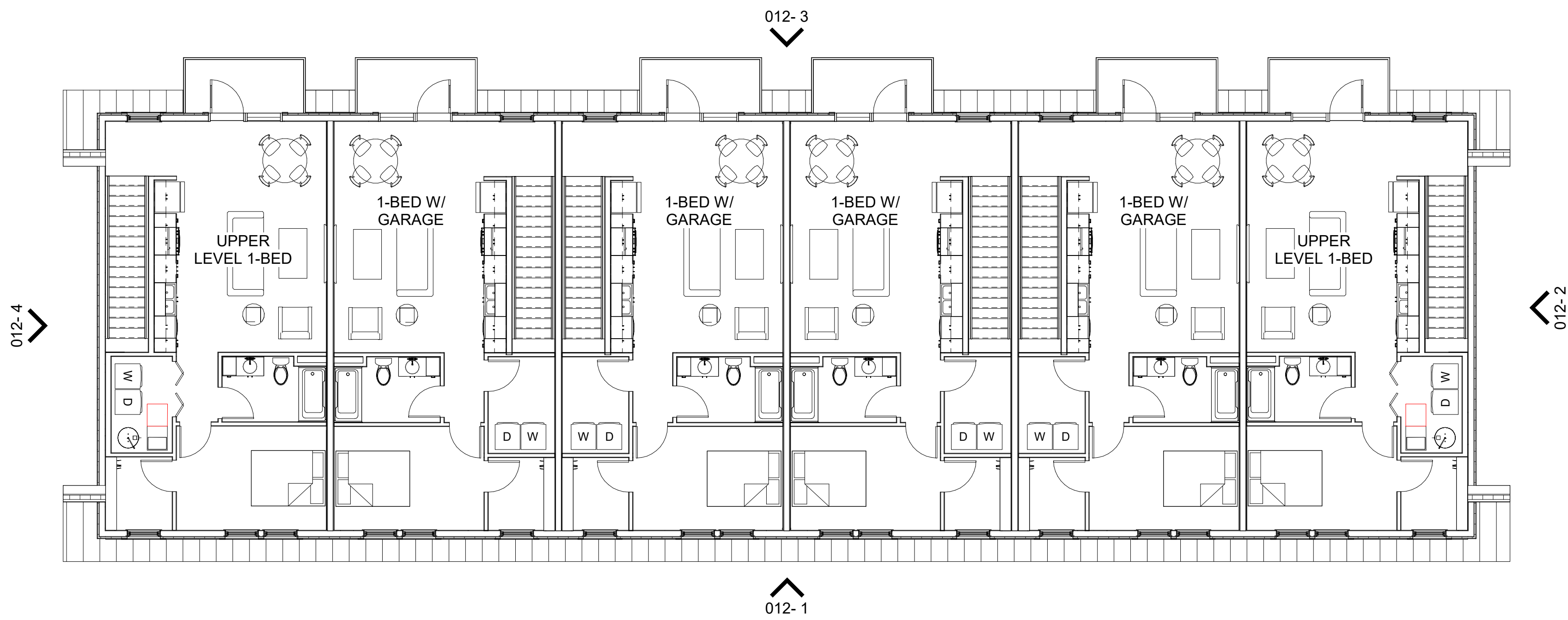
2 BUILDING 2 - LEVEL 2 1/8" = 1'-0"
