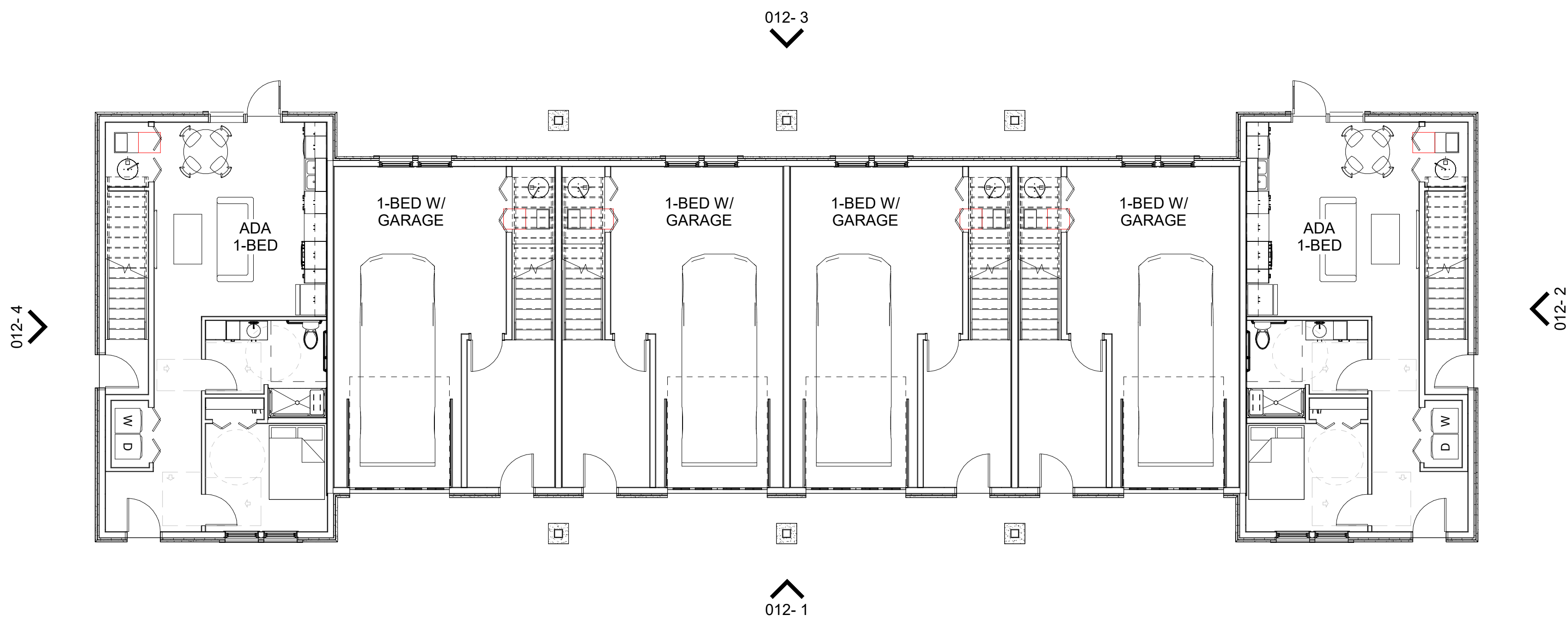
1 BUILDING 2 - LEVEL 1 1/8" = 1'-0"
